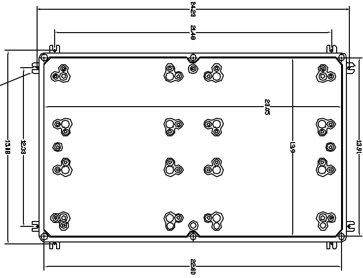
FRONT VIEW COVER REMOVED
