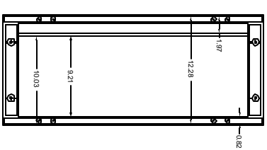
INNER DOOR PANEL
