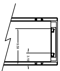
FIXED MOUNTING FRAME
