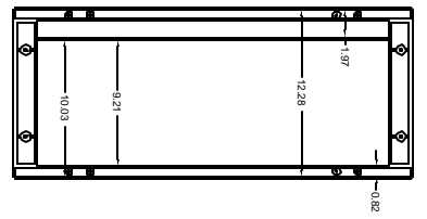
INNER DOOR PANEL
