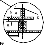
INNER DOOR PANEL
