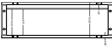
INNER DOOR PANEL
