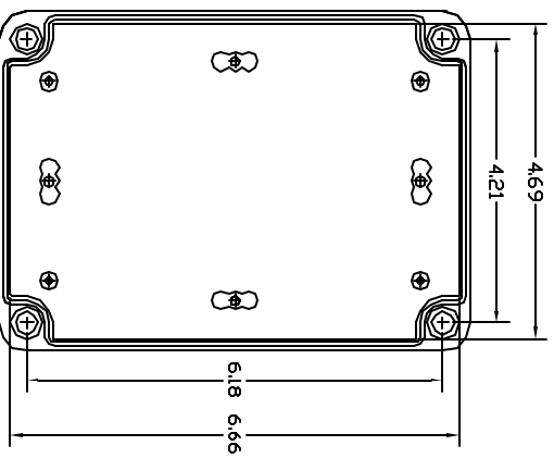
FRONT VIEW COVER REMOVED
